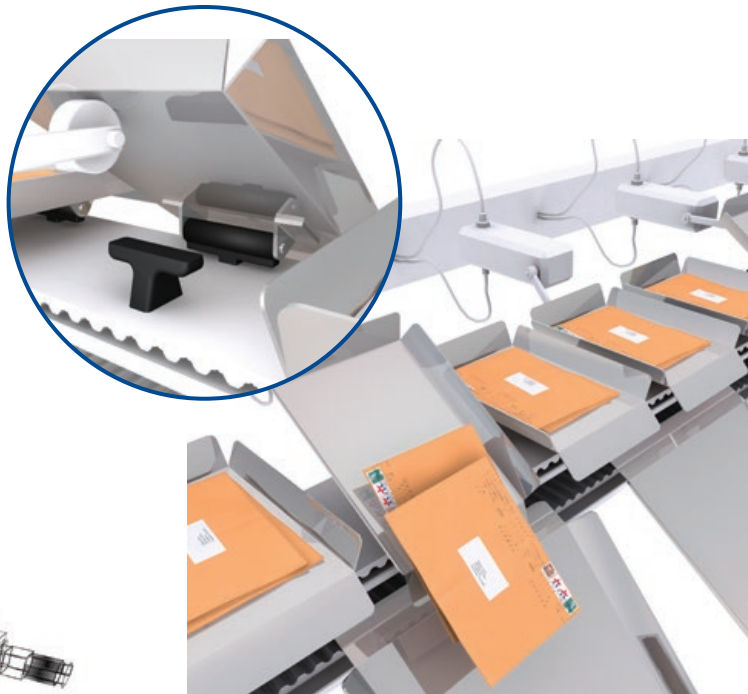
Custom profiles are used for pins and rests on a tilt-tray mail sorting machine.
